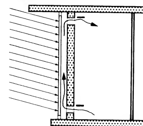
⑪ Winter day: incident solar radiation heats the air between the pane and the Trombè wall; room air is circulated through the lower and upper flaps and thus heated
